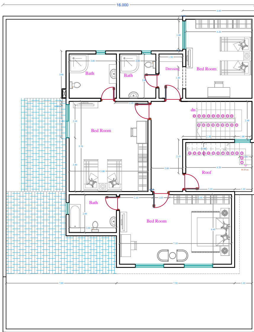
First Floor Plan Building Area = 146 m 2
