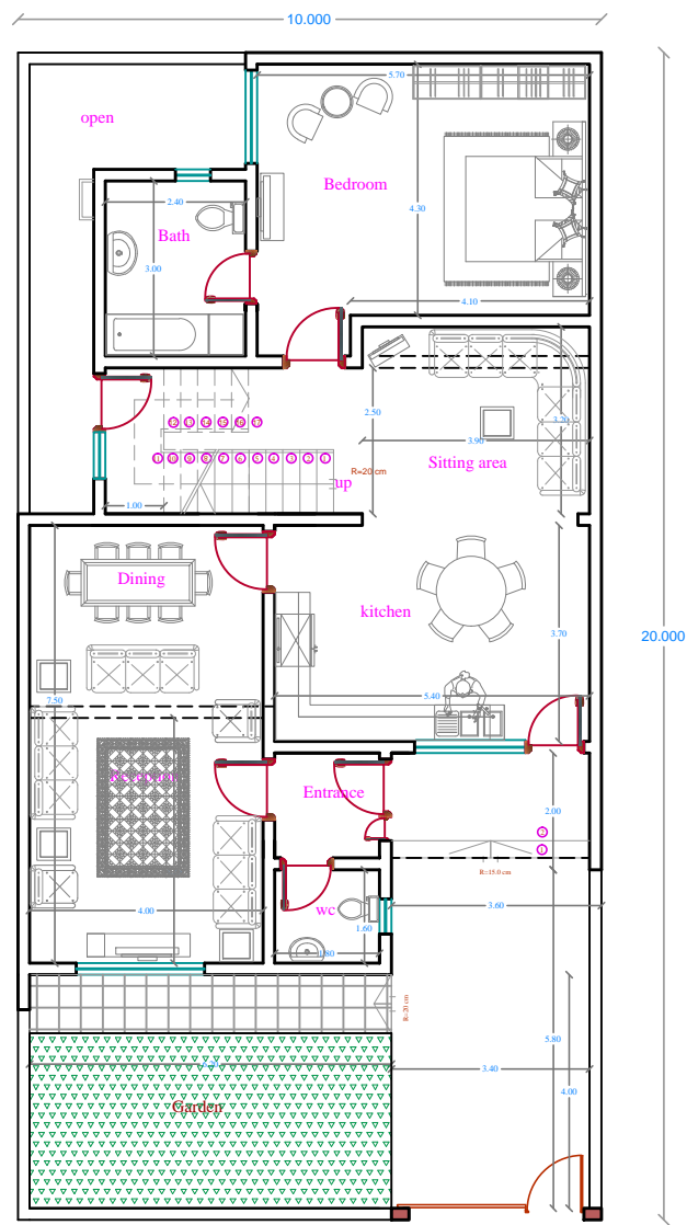
Ground Floor Plan Building Area = 136 m 2
