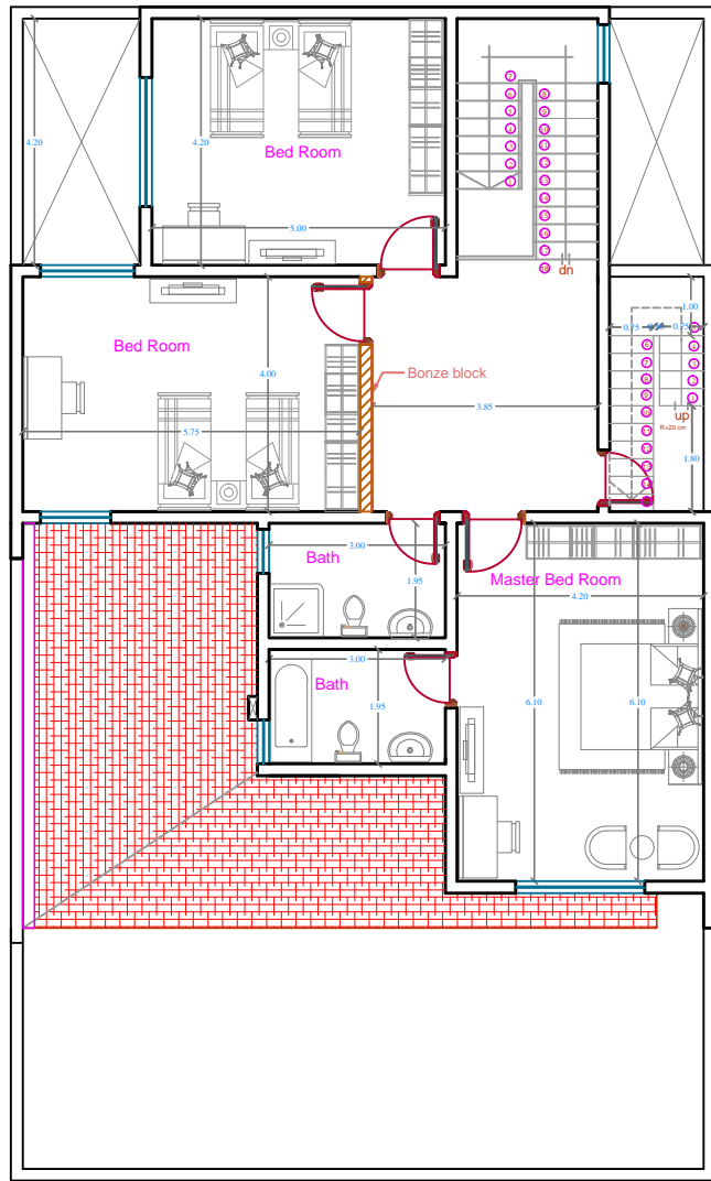
First Floor Plan Building Area = 123 m 2
