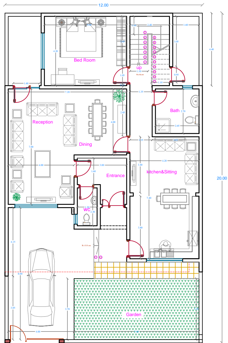
Ground Floor Plan Building Area = 170 m 2
