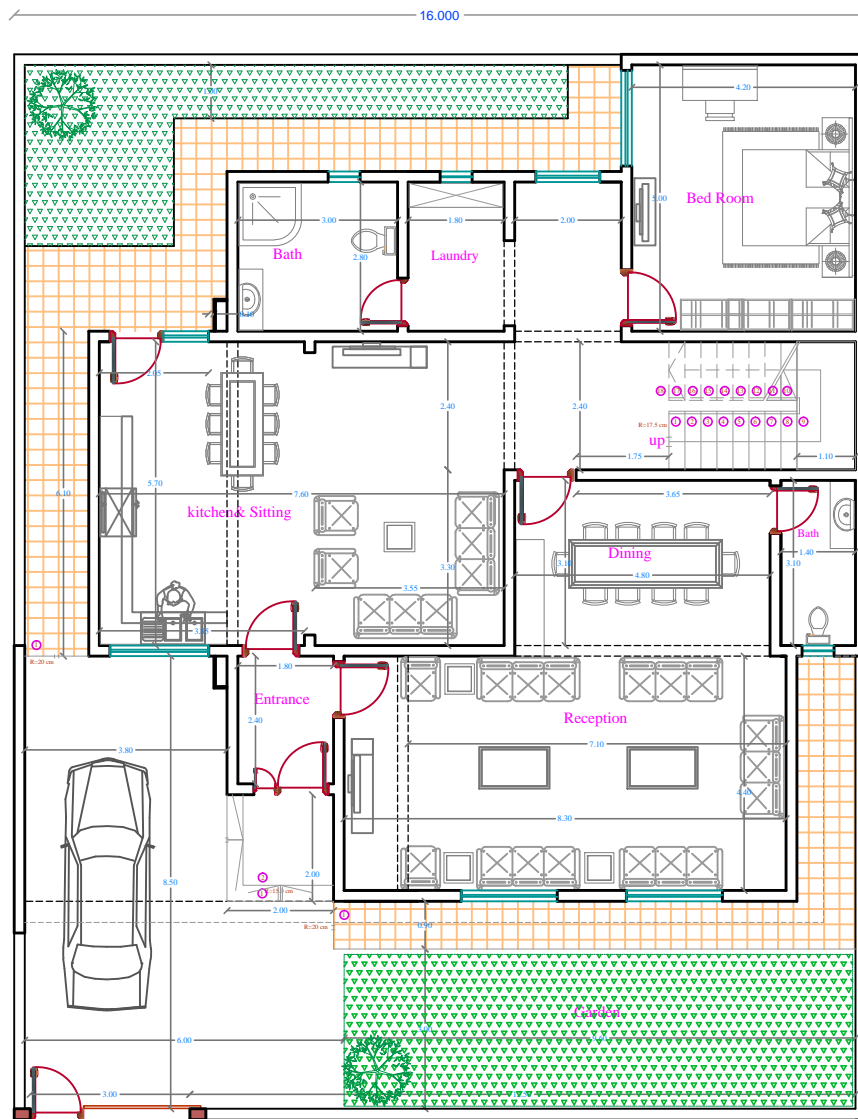
Ground Floor Plan Building Area = 203 m 2
